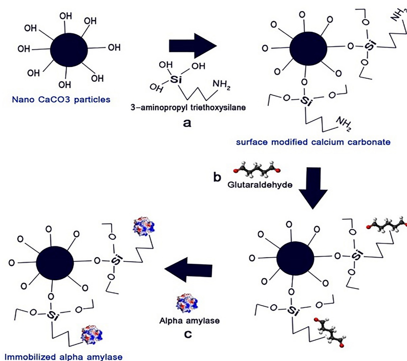
Figure 5. Procedure involved in immobilization of alpha-amylase by covalent attachment method. (a) preparation of functional group on the surface of nano CaCO 3 particles; (b) Modified nano CaCO 3 particles preparation by glutaraldehyde; (c) covalent attachment of the enzyme reactive functional groups (-NH 2 ) and the modified nano CaCO 3 particles.
