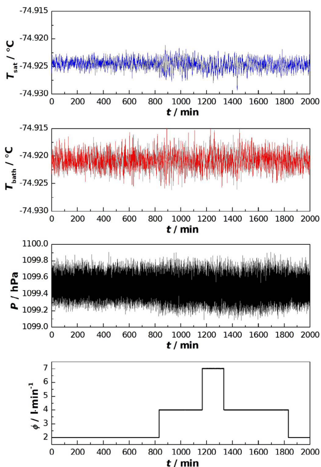
Figure 6. Saturated gas temperature T_{\text{sat}} stability at a saturator temperature T_{\text{bath}} of -75 °C, a pressure value of 1100 hPa and a flow rate including between 2 \text{l}\cdot\text{min}^{-1} and 7 \text{l}\cdot\text{min}^{-1} . The T_{\text{sat}} stability results in being better than 0.006 °C.
