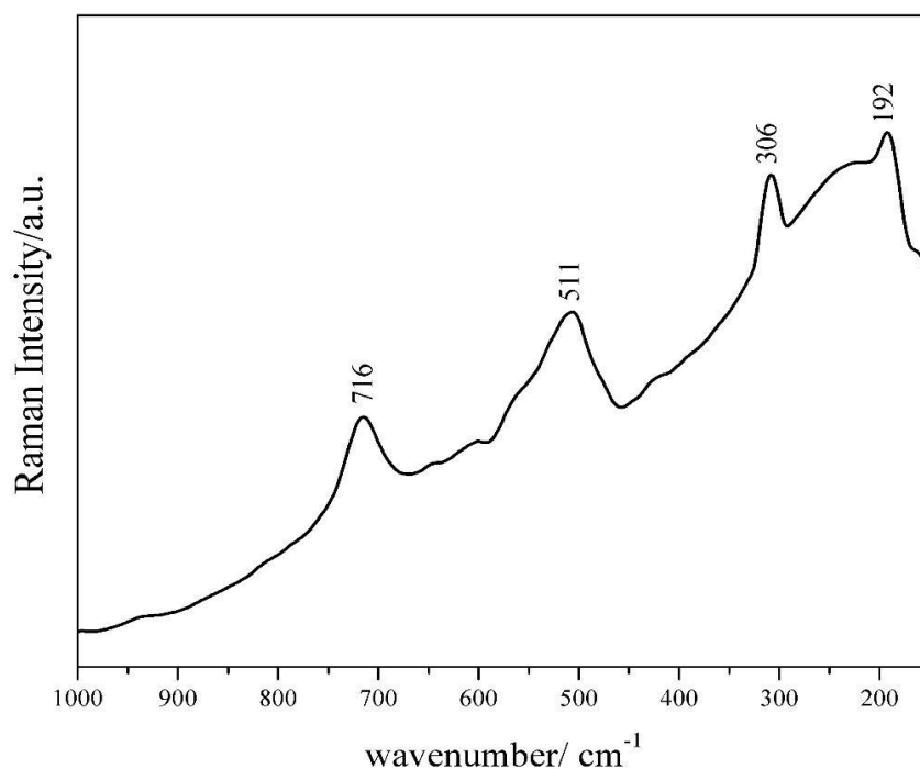
Fig. 2. Raman spectra of barium titanate nanoparticles (BaTiO 3 NPs)
