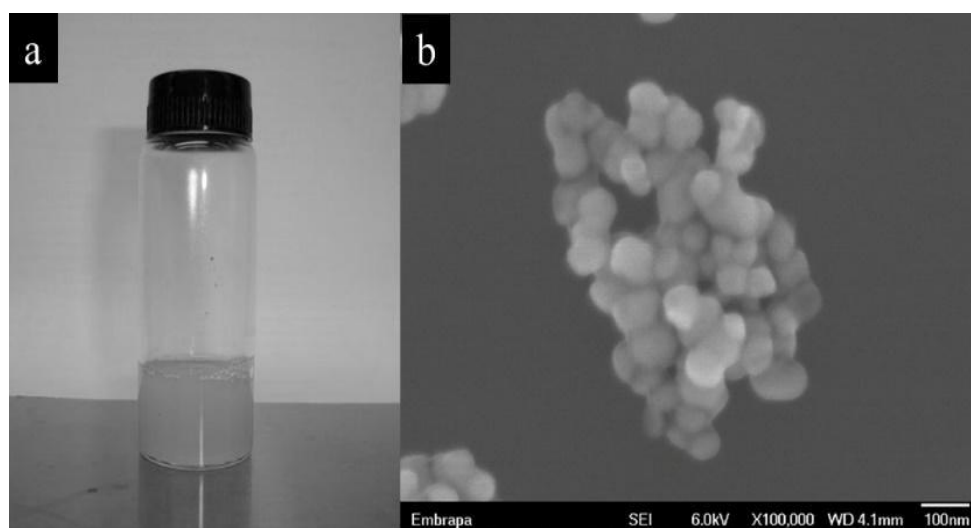
Fig. 1. (a) Suspensions of barium titanate nanoparticles (BaTiO 3 NPs) in Dulbecco's Modified Eagle Medium (100 \mu g mL -1 ). (b) Scanning electron microscopy (SEM) images of BaTiO 3 NPs. Scale bar =100 nm
