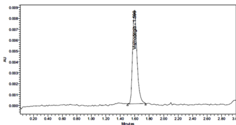
Fig. 5. LOQ Chromatogram of VMD
