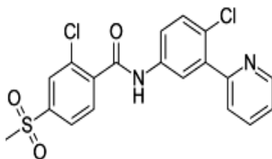
Fig. 1. Structure of VMD
