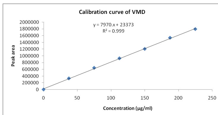
Fig. 3. Linearity curve of VMD
