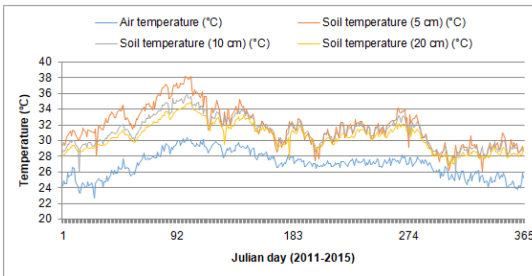
Fig. 3. Julian day graph (2011 to 2015) - Daily average air temperature and soil temperature at 5cm, 10cm and 20cm depths of the representative block (CBE); Soil type-Sandy clay loam
