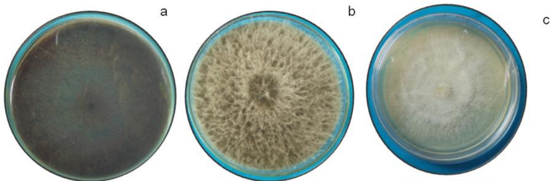
Fig. 2. Pathogens isolated from infected mulberry root samples a. Macrophomina phaseolina b. Lasiodiplodia theobromae c. Fusarium sp.
