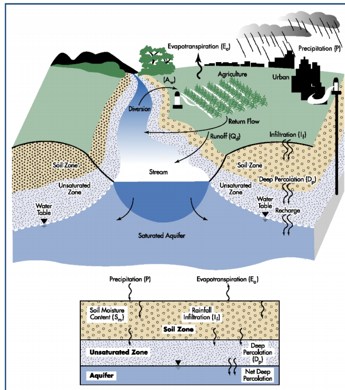
Fig. 8. Rainfall, runoff, soil moisture accounting and unsaturated zone simulation components
