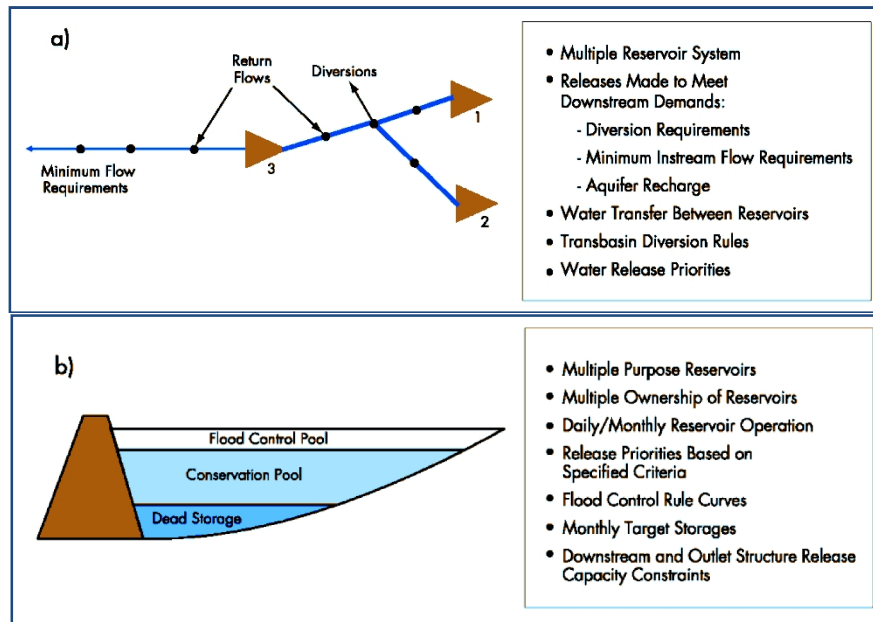
Fig. 11. River/reservoir operations simulations
