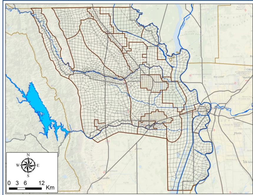
Fig. 19. Finite element grid for Yolo county model
