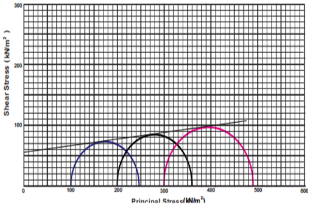
Fig. 4. Graphical presentation showing shear stress against principal stress at 4m depth
