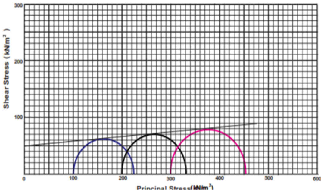
Fig. 5. Graphical presentation showing shear stress against principal stress at 2 m depth
