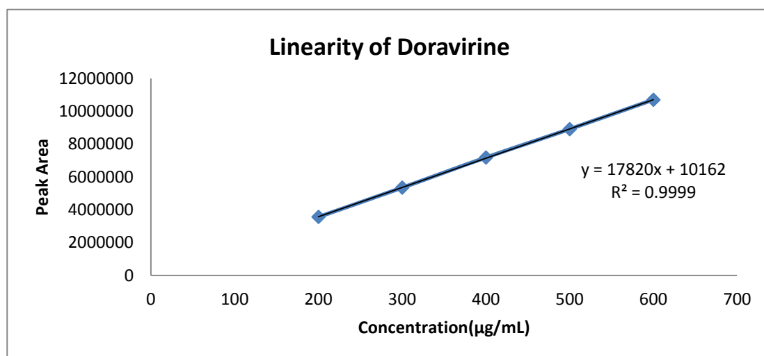
Fig. 3. Calibration curve of Doravirine
